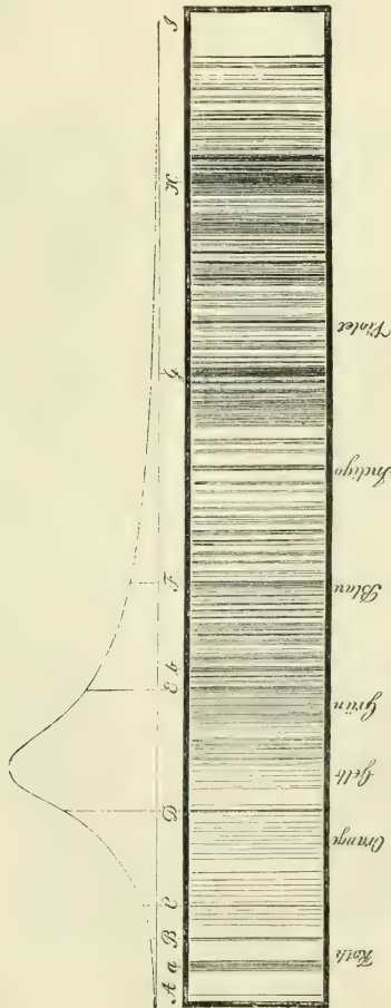
FIG. 12.—Copy of Fraunhofer's diagram of the lines in the solar spectrum with his original lettering of the principal lines.
